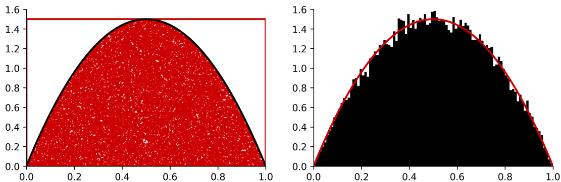
Figure 2.6: On the left, we plot the accepted samples (scattered) under the curve. On the right, we describe the histogram of x -marginal of these samples (so we just keep the first dimension of the two dimensional array).
