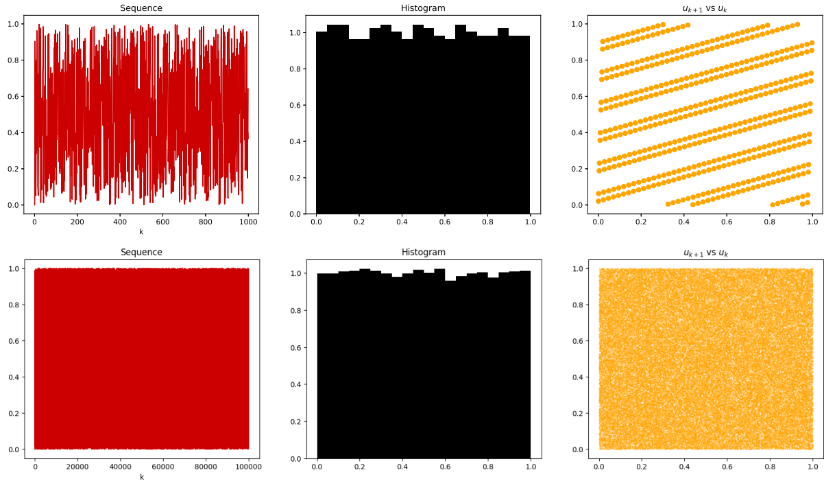
Figure 2.1: Top Left: Samples generated by an LCG with parameters m = 2048 , a = 43 , b = 0 , x_0 = 1 . Top Middle: The histogram of the samples showing that it conforms the uniform distribution. Top Right: However, plotting (u_k, u_{k+1}) pairs shows that the samples are not random enough . Bottom Left: Samples generated by an LCG with parameters m = 2^{32} , a = 1664525 , b = 1013904223 . Bottom Middle: The histogram of the samples showing that it conforms the uniform distribution. Bottom Right: Plotting (u_k, u_{k+1}) pairs shows that the samples do not look nonrandom.
