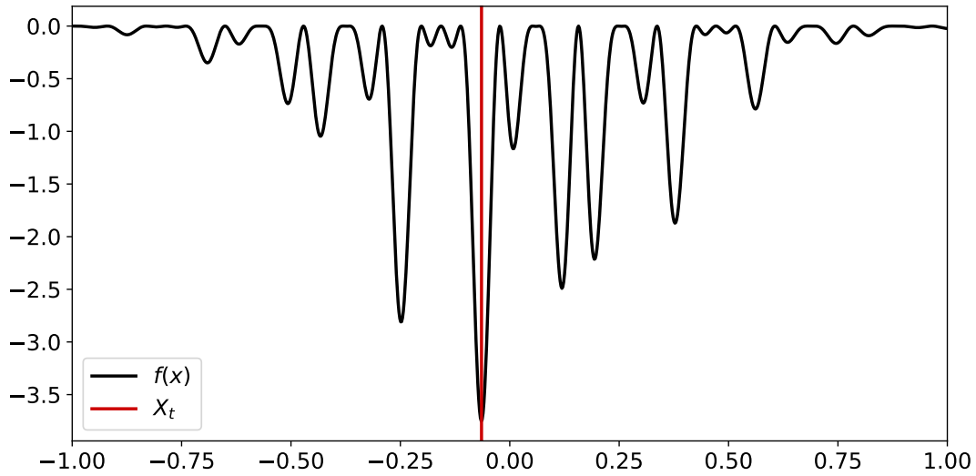
Figure 5.6: Simulated annealing for the function in Eq. 5.10. The red line shows the final estimate of SA algorithm.
