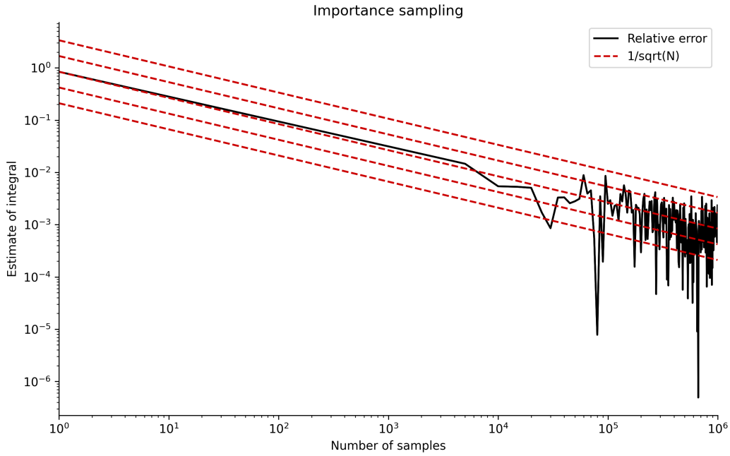
Figure 4.8: The importance sampling estimator \hat{\varphi}_{\text{IS}}^N is plotted against the number of samples N for the example in in Fig. 4.7, for \varphi(x) = x^2 . This demonstrates that the random error in the IS case also satisfies \mathcal{O}(1/\sqrt{N}) convergence rate.
