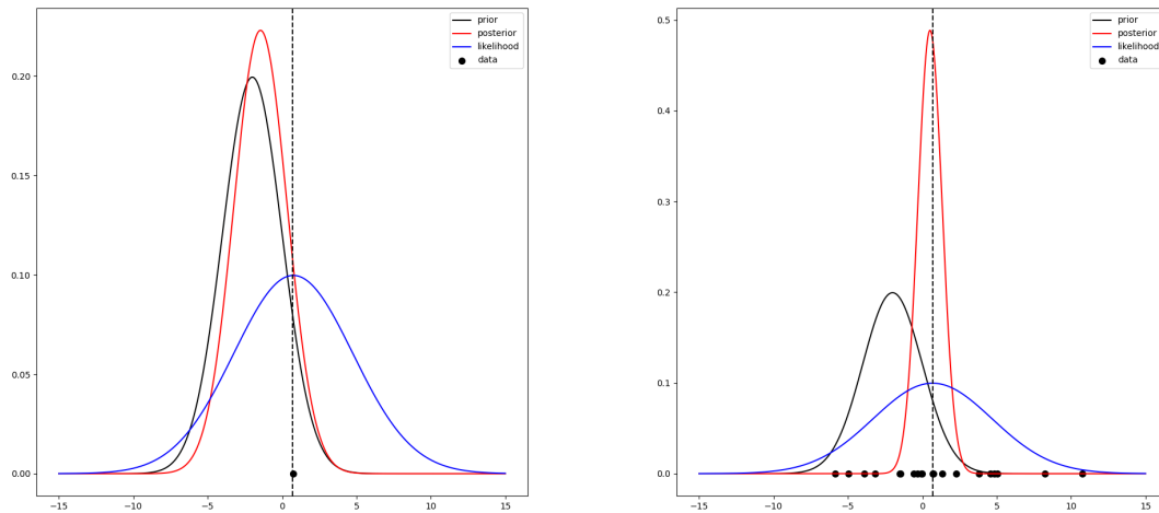
Figure 3.5: Bayes update for conditionally independent observations.
